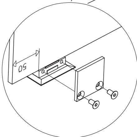
Floor Bracket
